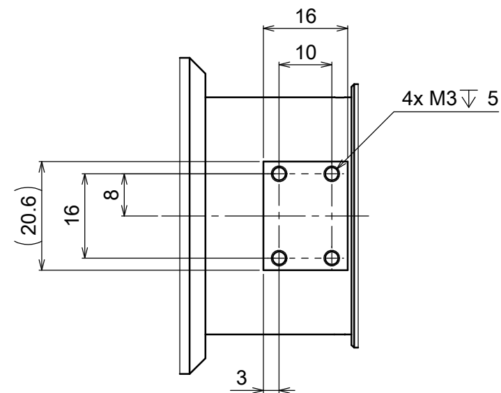
VIEW A
