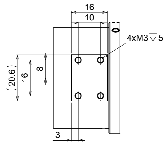
VIEW A
